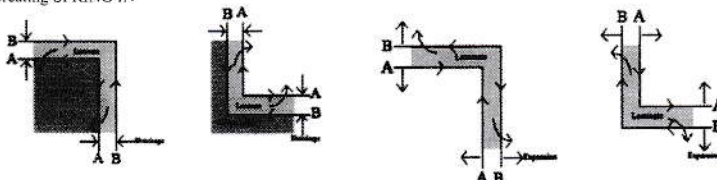
The Effect of Warpage & Spring Forward of Composite tools
