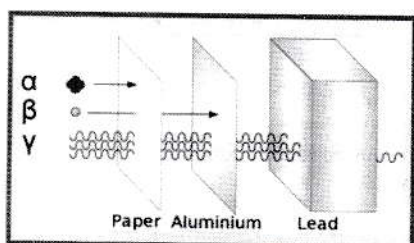
Figure 1: Comparison between various radiation types
